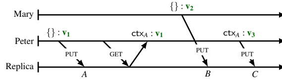
Fig. 1: Example execution for one key: Peter writes a new value \mathbf{v}_1 (A), then reads from Replica ( \text{ctx}_A ). Next, Mary writes a new value \mathbf{v}_2 (B) and finally Peter updates \mathbf{v}_1 with \mathbf{v}_3 (C).
